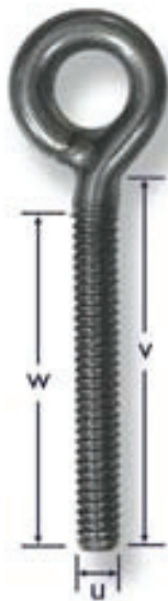
Eye Bolts
